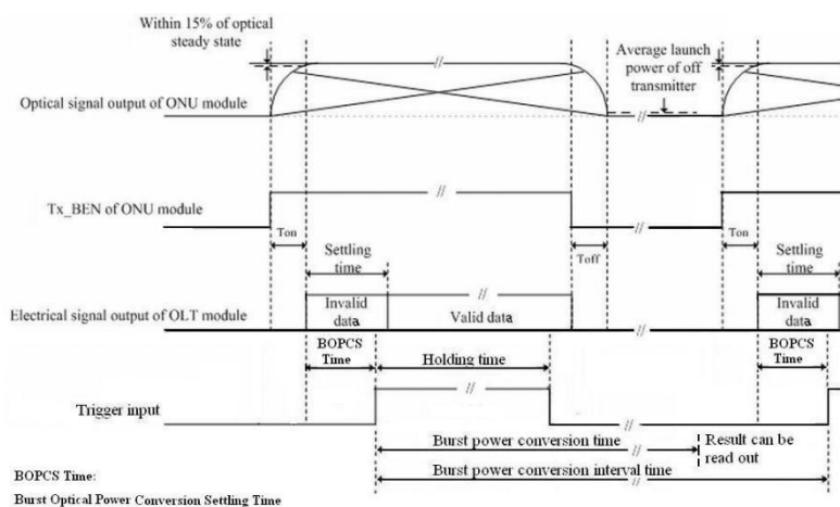
Fi7 Trigger sequence definition in GPON system
