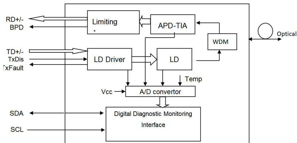
Fig 1 Transceiver Block Diagram
