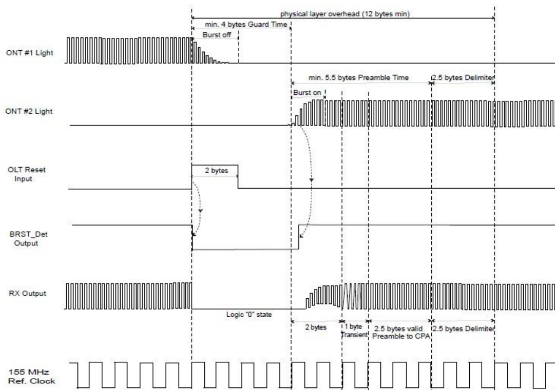
Fig6 Time parameter definition in GPON system
