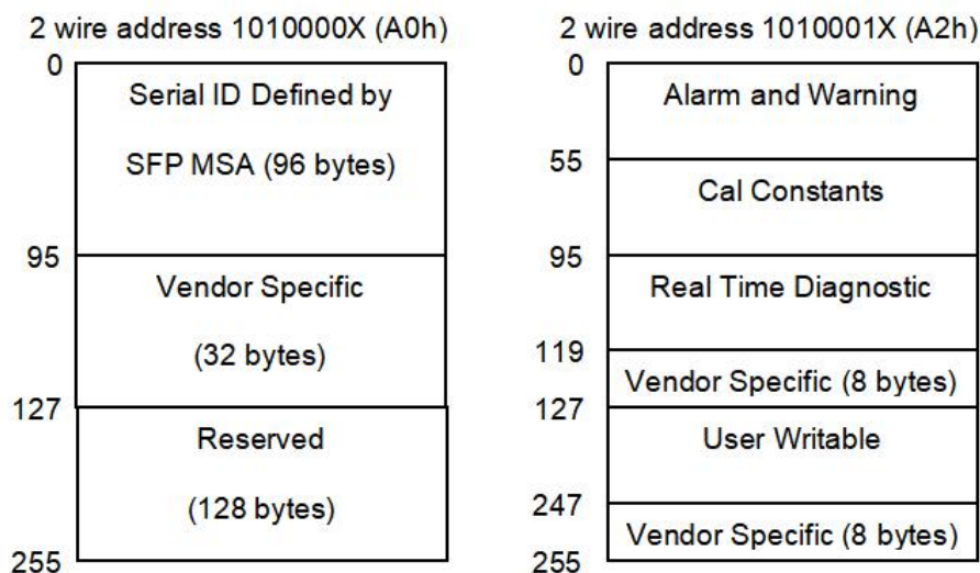
Fig 2 EEPROM Information
